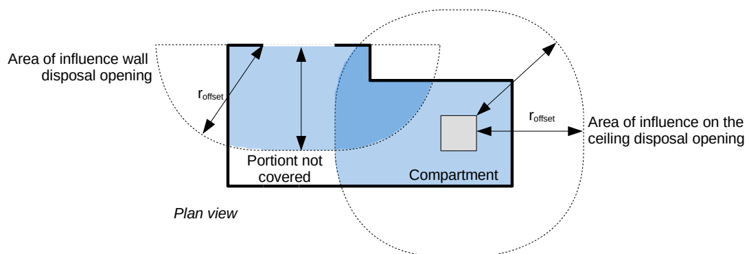
Image 14: Verification of the uniform distribution in plan in the facility of the venting opening
